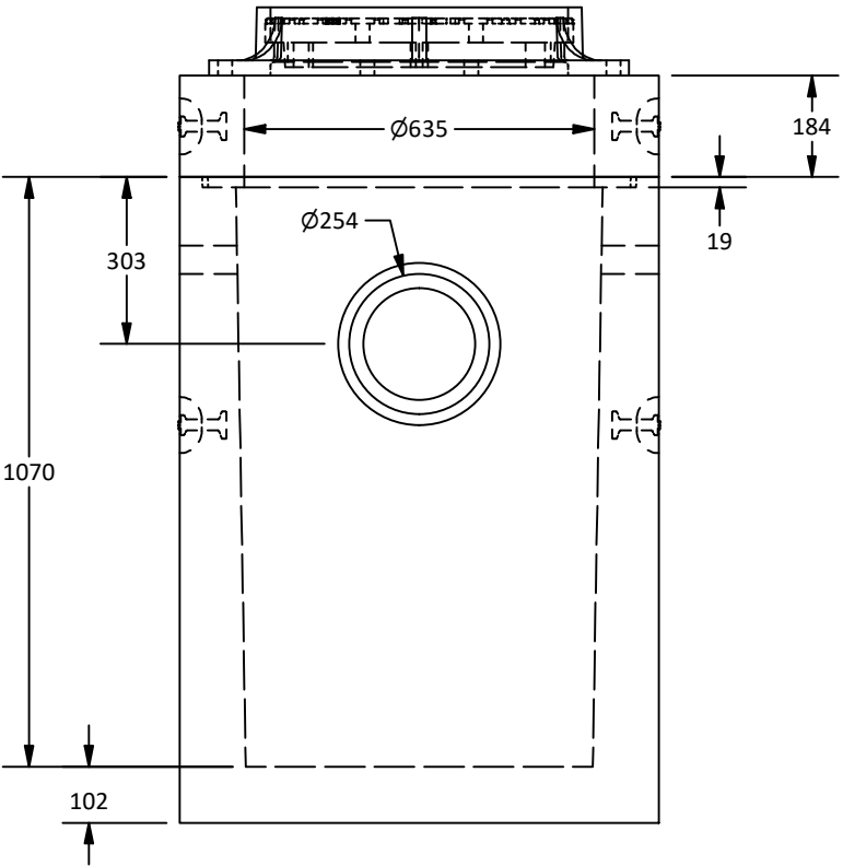
East View
