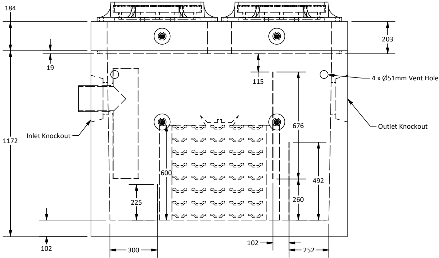
Elevation View
