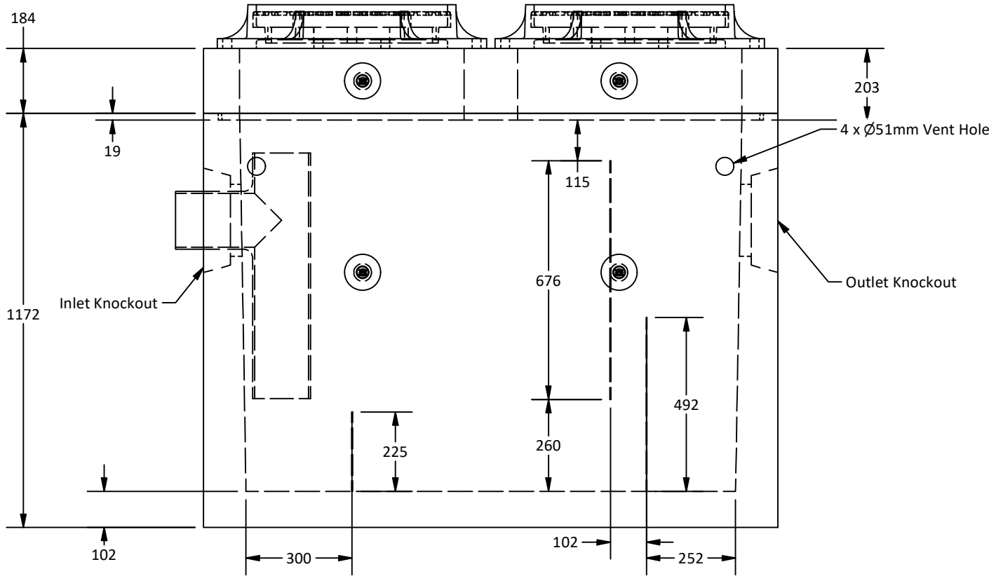
Elevation View
