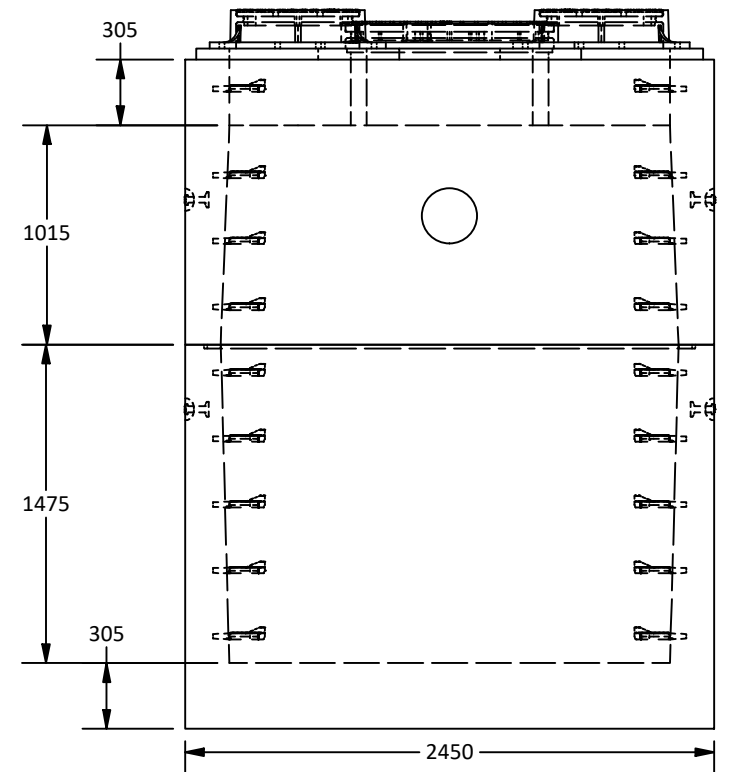
East View
