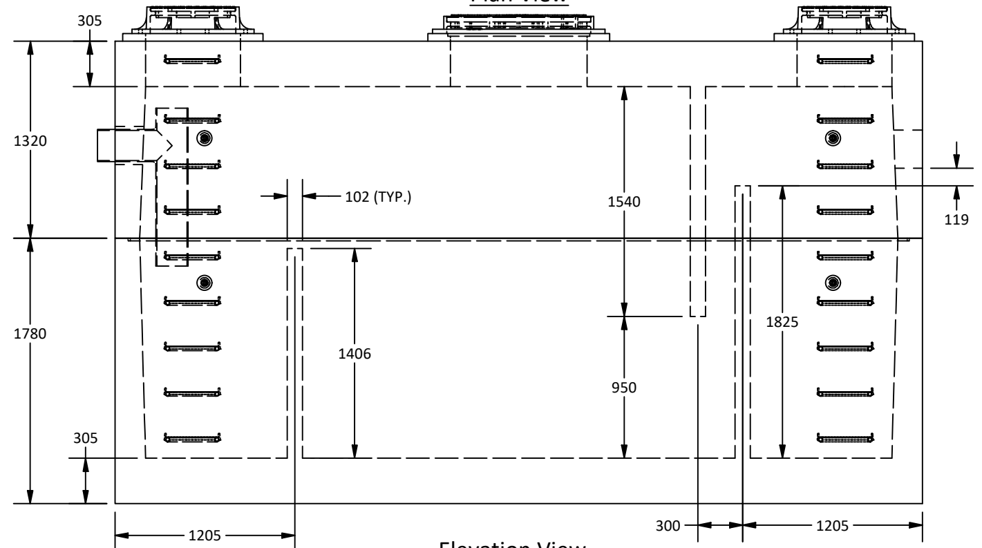
Elevation View
