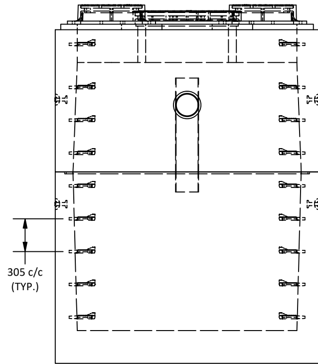
West View
