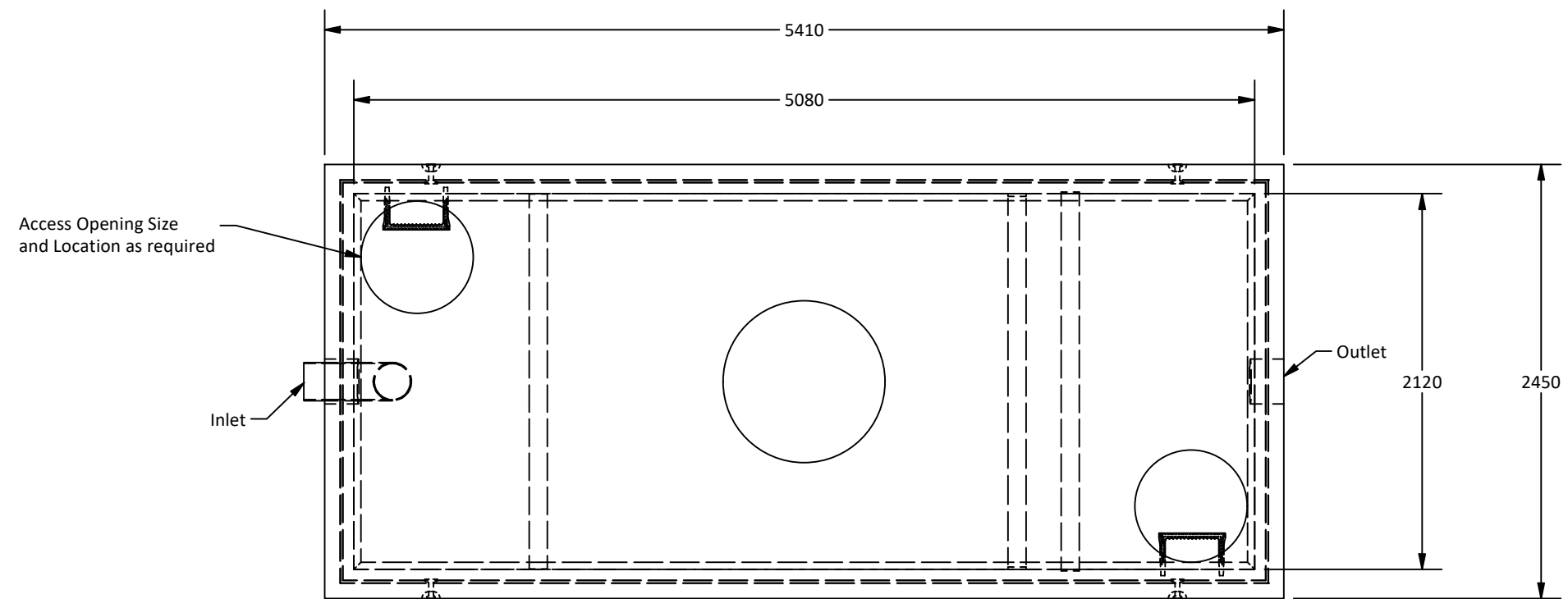
Plan View
