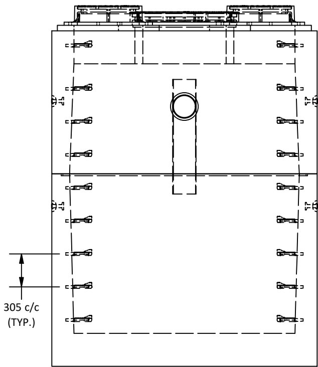
West View
