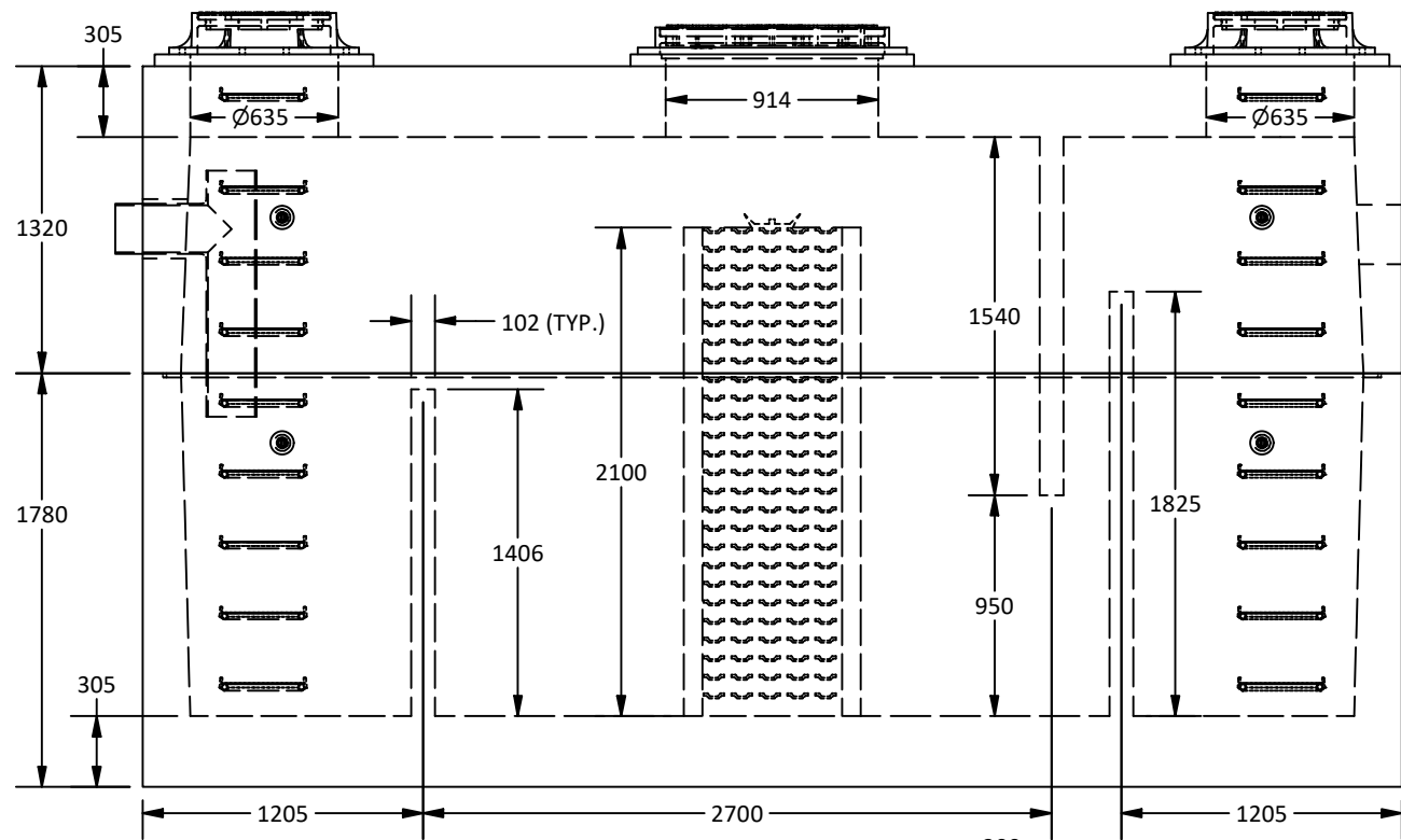
Elevation View
