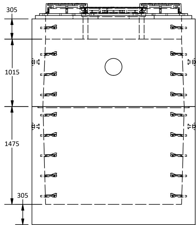
East View
