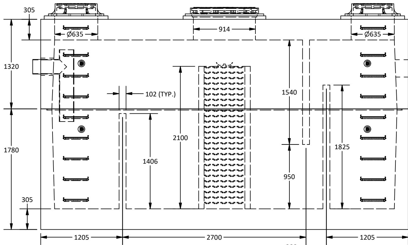
Elevation View
