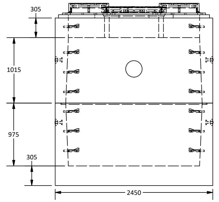
East View
