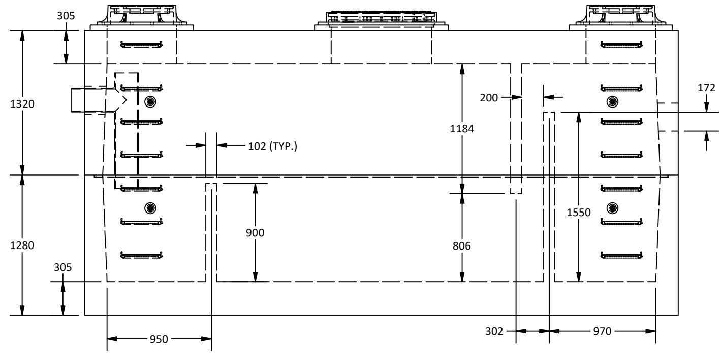
Elevation View
