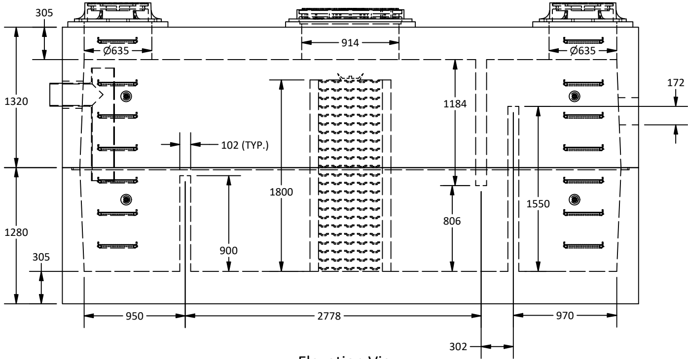
Elevation View
