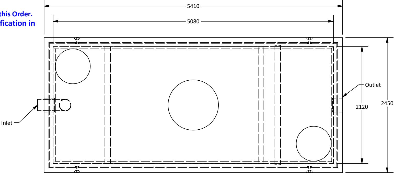
Plan View
