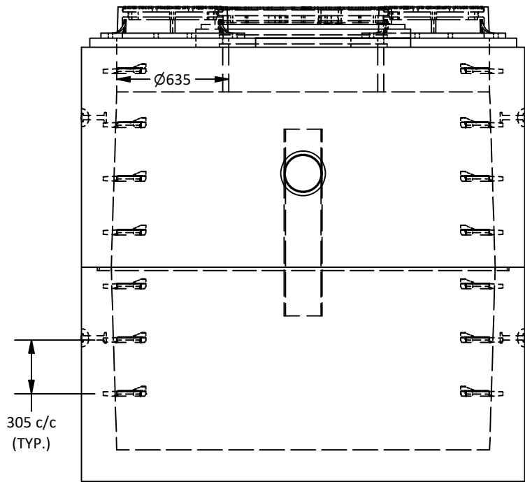
West View
