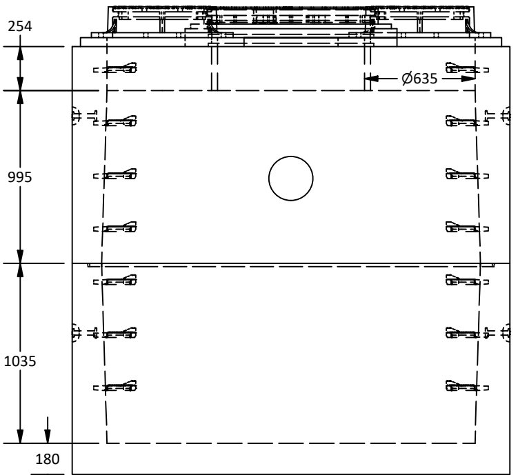
East View
