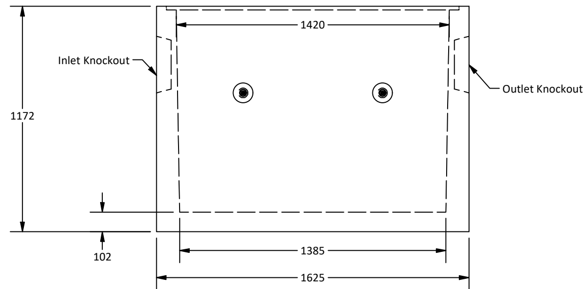
Elevation View
