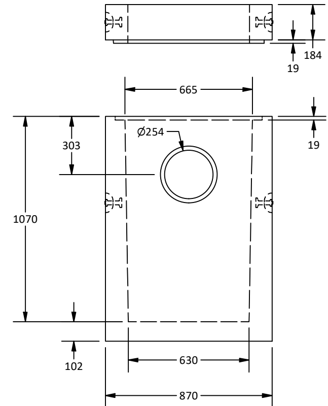
East View
