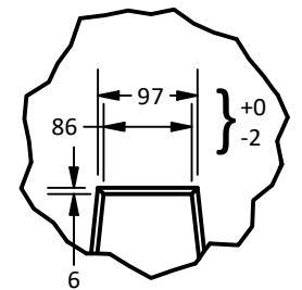
Detail D Scale 1:8
