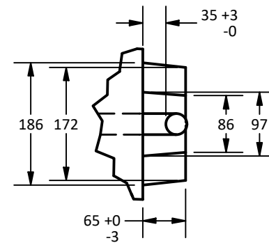
Detail C Scale 1:8
