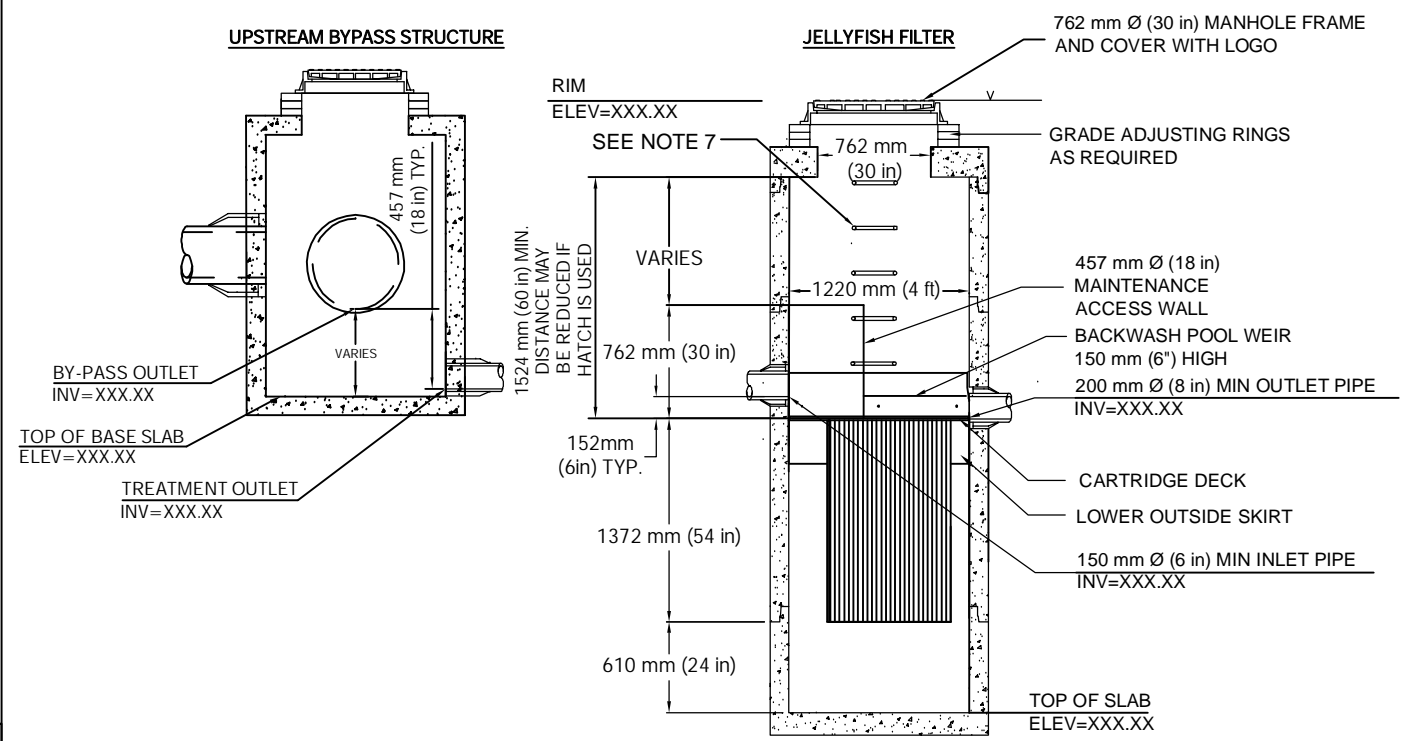
CROSS SECTION 1-1
