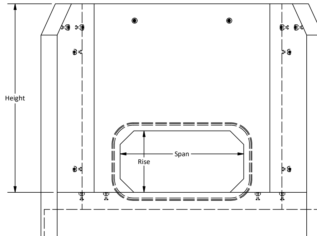
Elevation View
