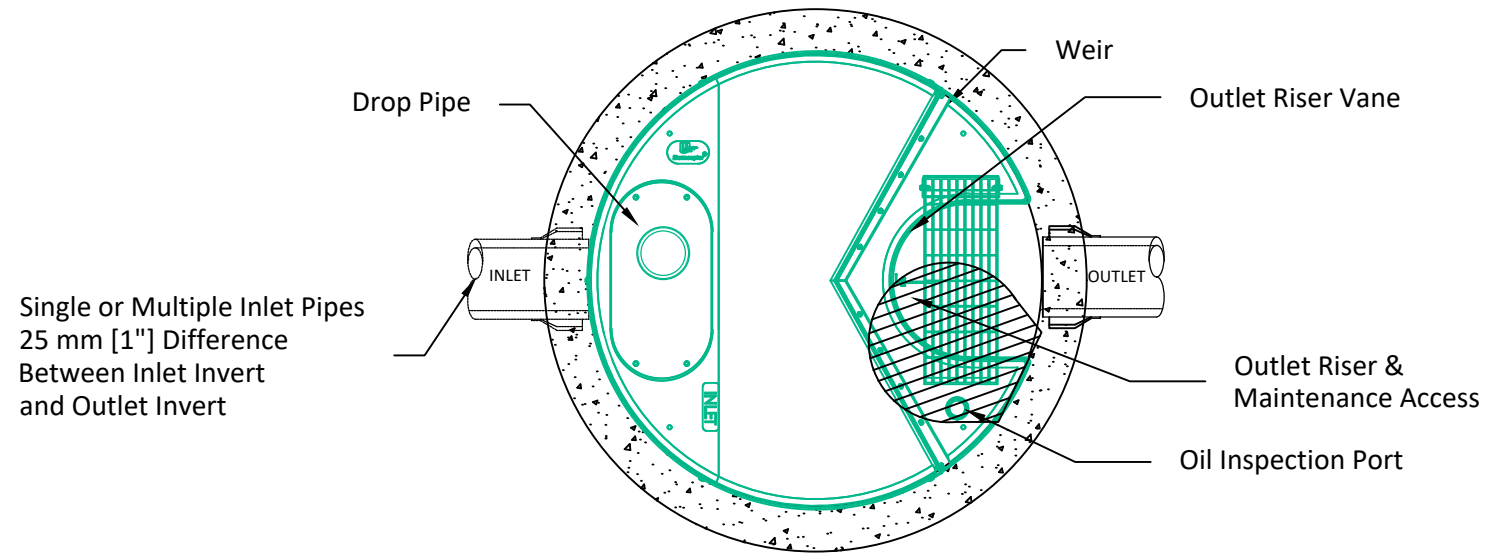
Plan View
