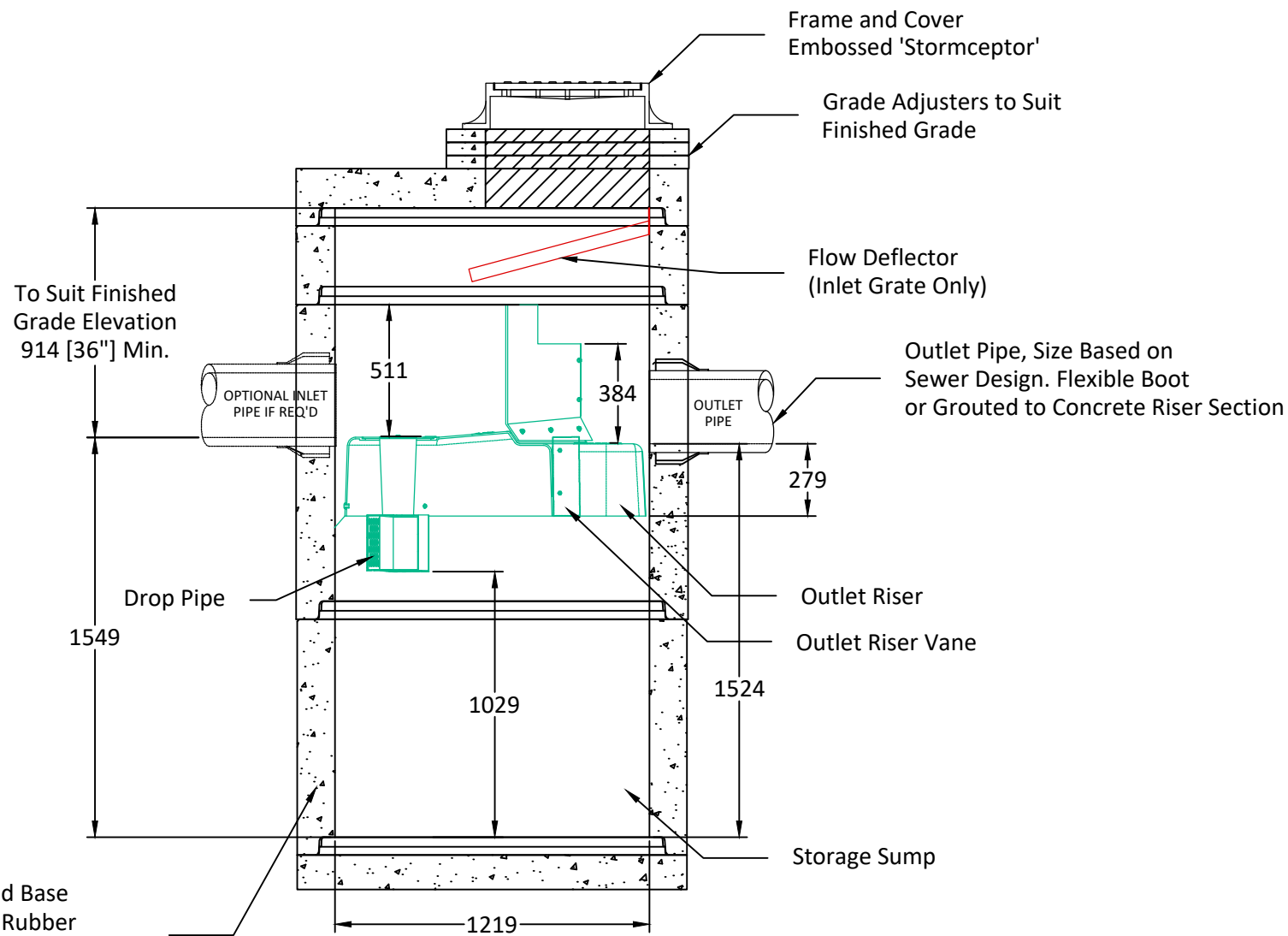
Elevation View
