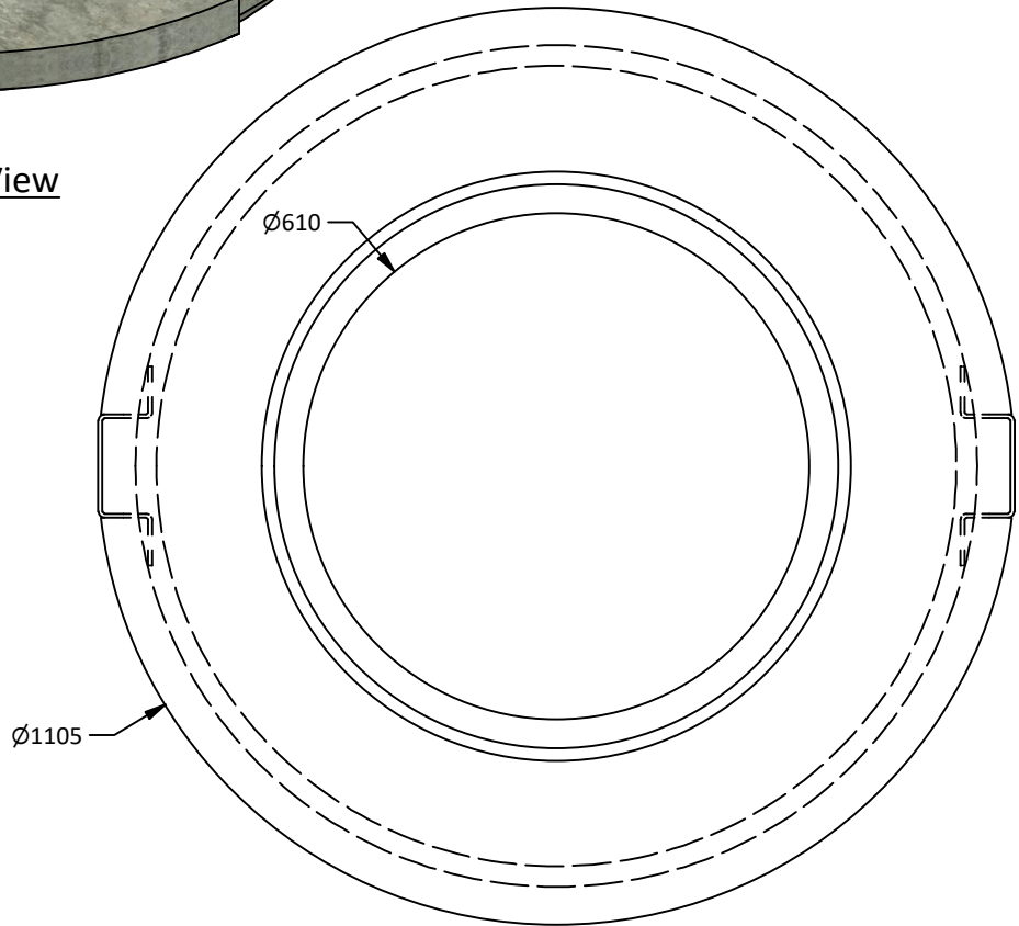
Plan View
