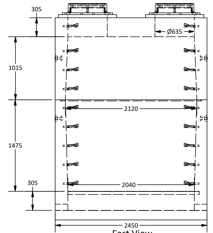
East View
