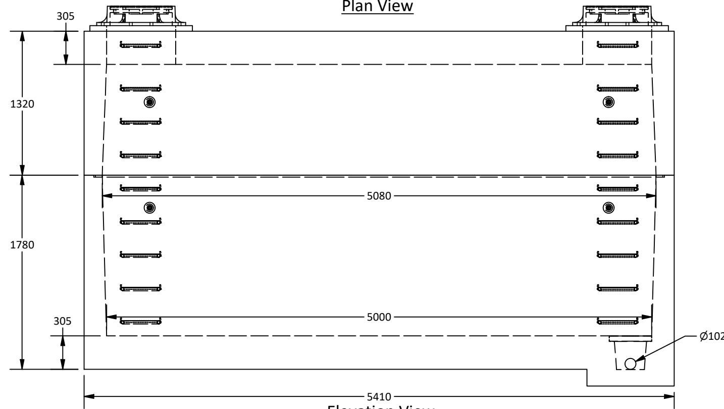
Elevation View
