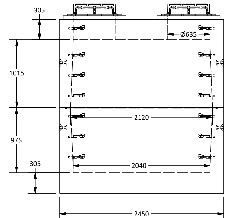
East View
