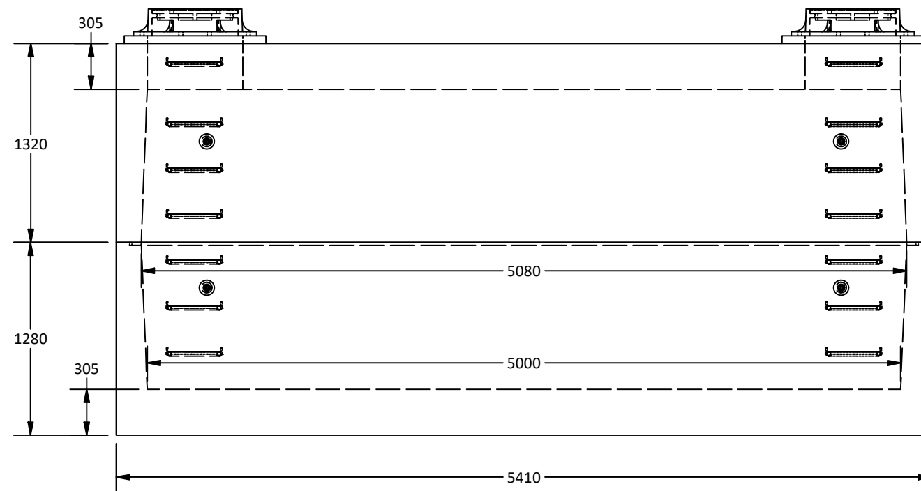
Elevation View
