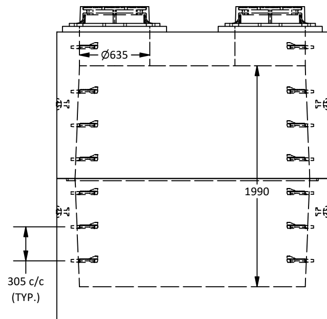
West View
