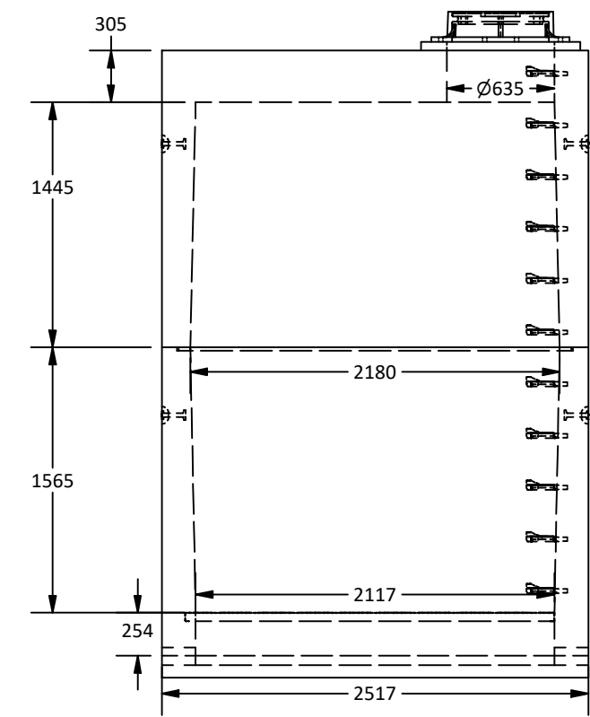
East View
