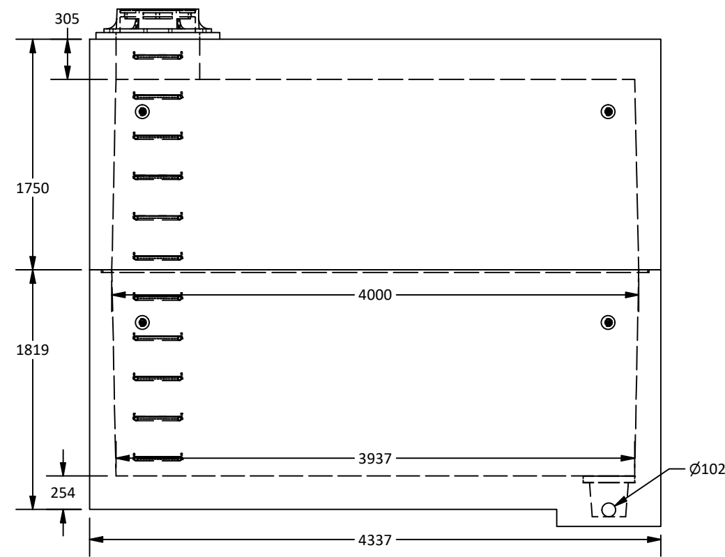
Elevation View
