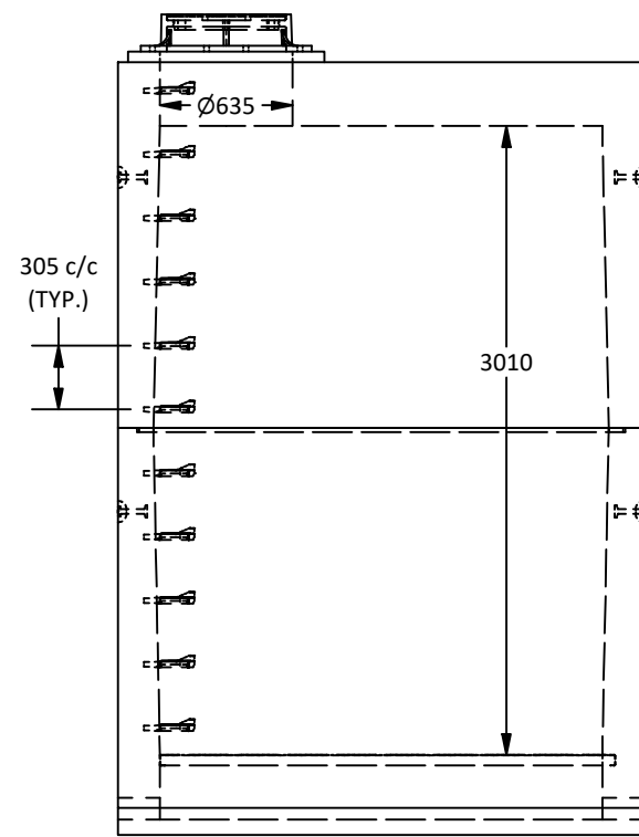
West View
