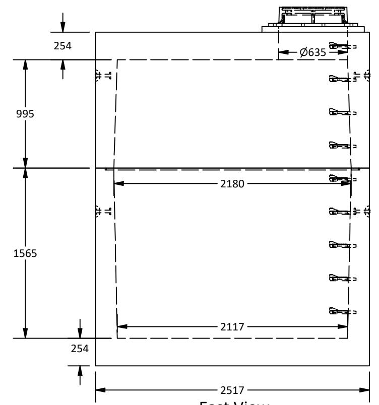
East View
