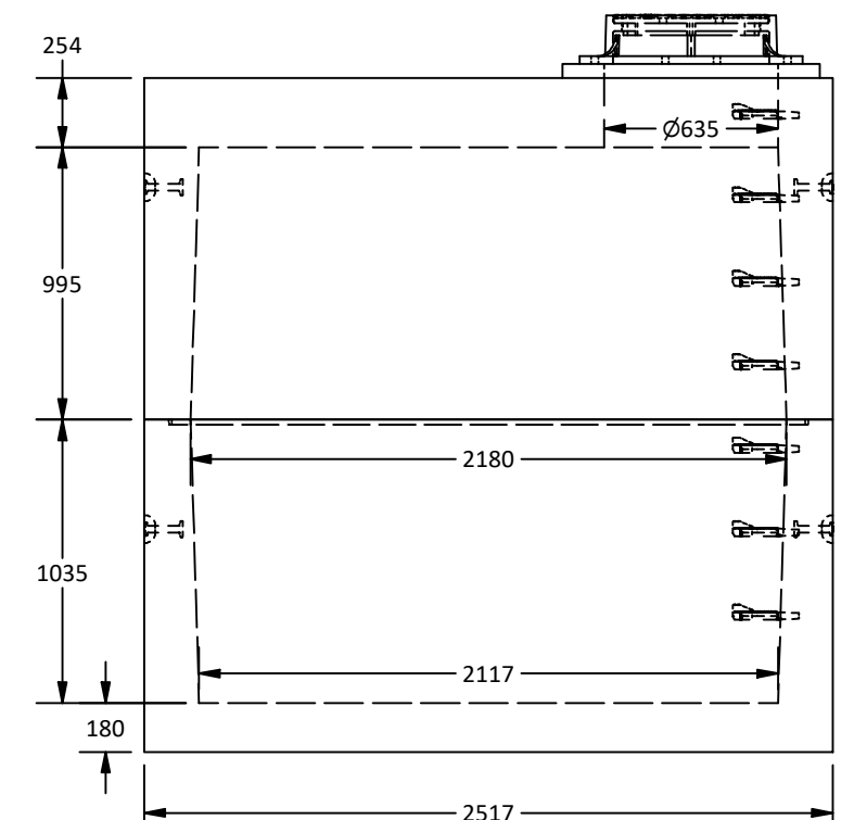
East View
