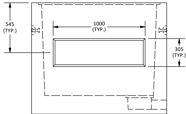
West View
