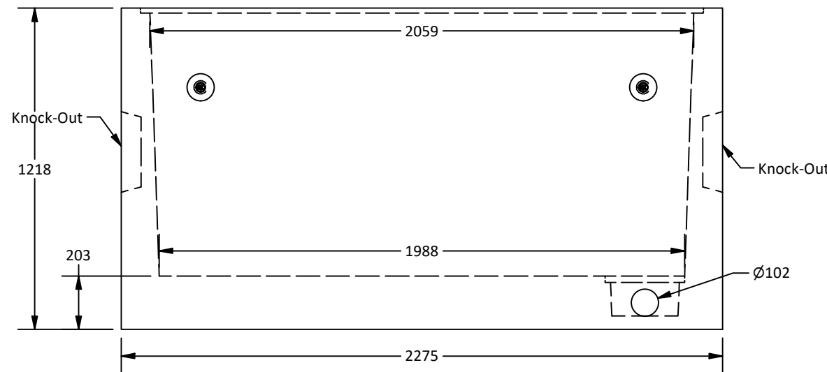
Elevation View
