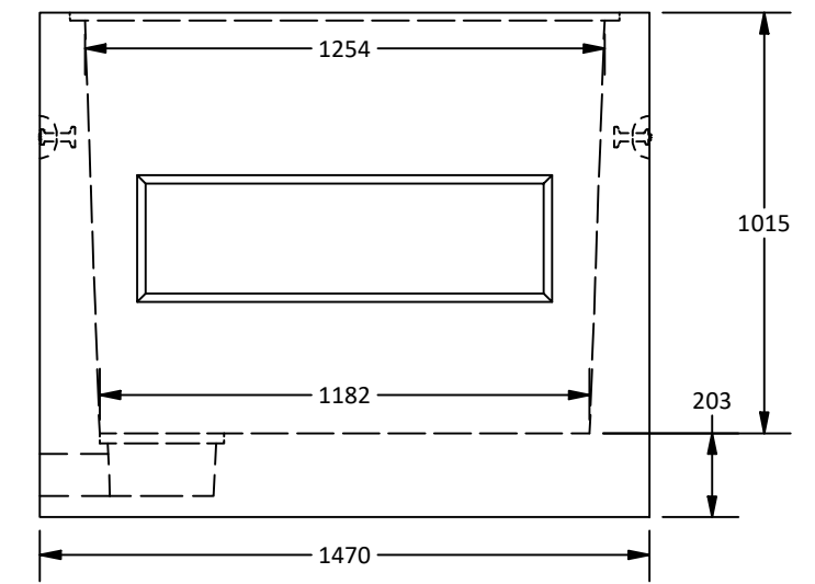
East View
