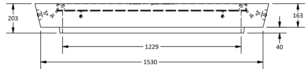
Elevation View
