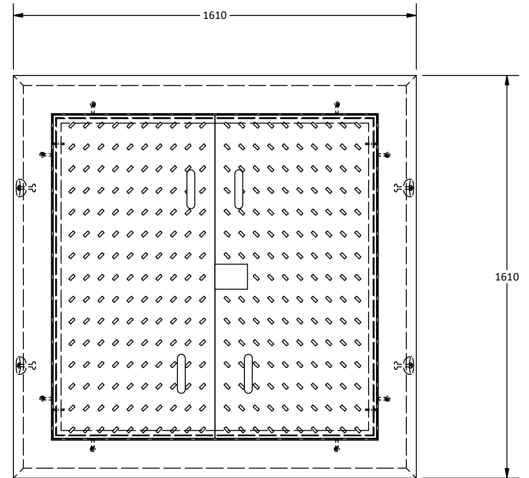
Plan View
