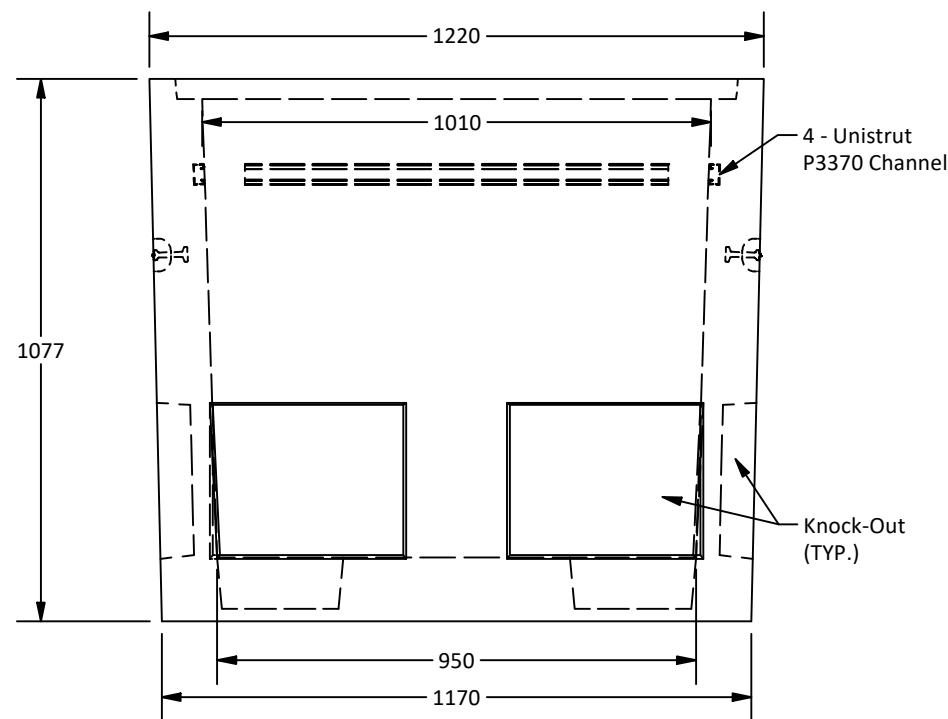
West View
