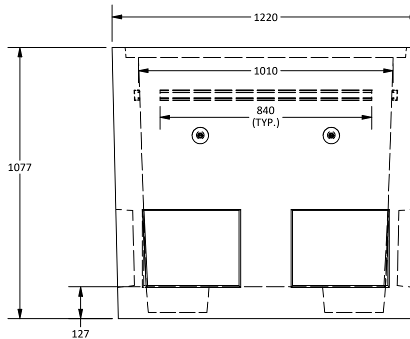
Elevation View
