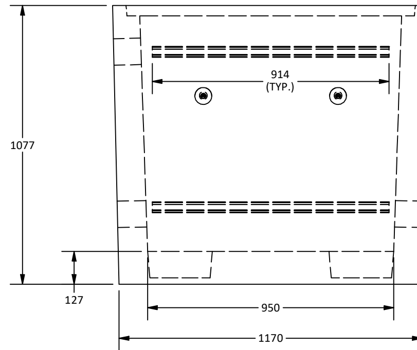
Elevation View
