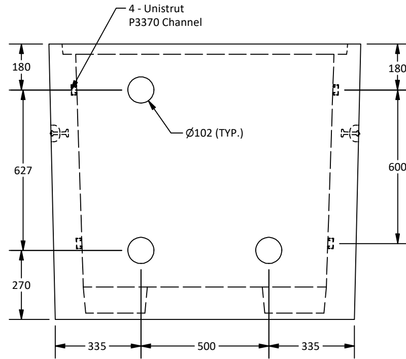
West View
